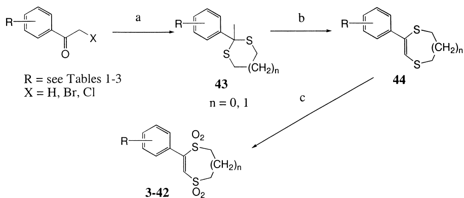
Scheme 1. Reagents and conditions: (a) \text{BF}_3 \cdot \text{OEt}_2 , \text{HSCH}_2(\text{CH}_2)_n\text{CH}_2\text{SH} ; (b) \text{Br}_2 or \text{NBS} ; (c) \text{H}_2\text{O}_2 , \text{HOAc} .
